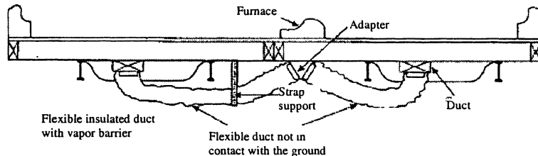
Figure A to §3285.606 – Crossover Duct Installation with Two Connecting Ducts.
